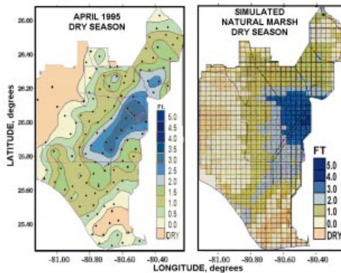
Figure 31. Comparison of current (left) vs. simulated natural marsh (right) water depths for the study area.
