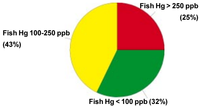
Figure 24. South Florida marsh (area-weighted) mosquitofish mercury concentration distributions.
