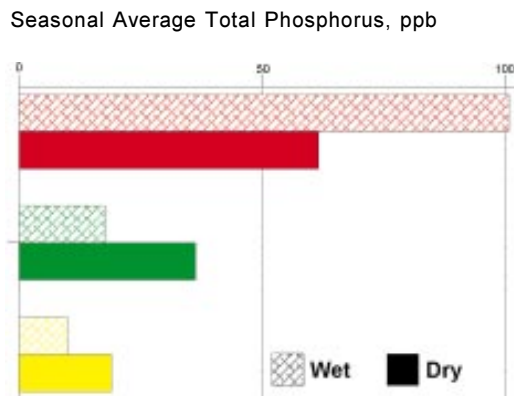
Figure 20. Water total phosphorus distribution in canals from north to south. Note: 50 ppb is the Phase I control target.
