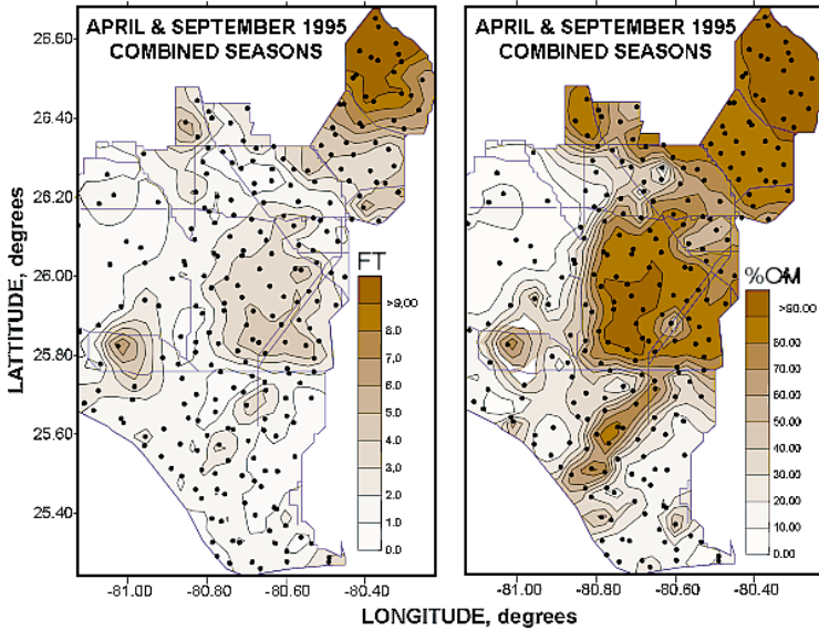
Figure 14. Thickness of the soil or peat deposits throughout the marsh.
