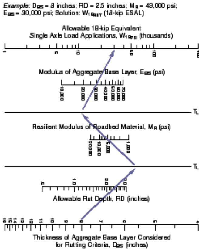
Figure 12: Design Chart for Aggregate-Surfaced Roads Considering Allowable Rutting. (39) From AASHTO Guide for Design of Pavement Structures . Copyright 1993, by the American Association of State Highway and Transportation Officials, Washington, D.C. Used by permission.
