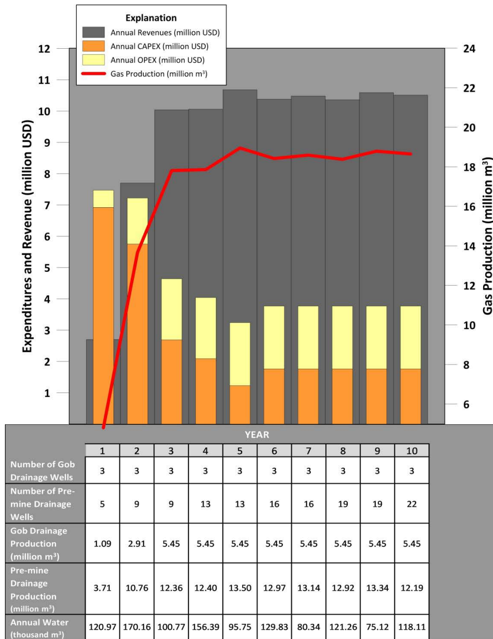
Figure 22: Gas Production, Expenditures and Revenues of the Proposed Methane Mitigation Plan
