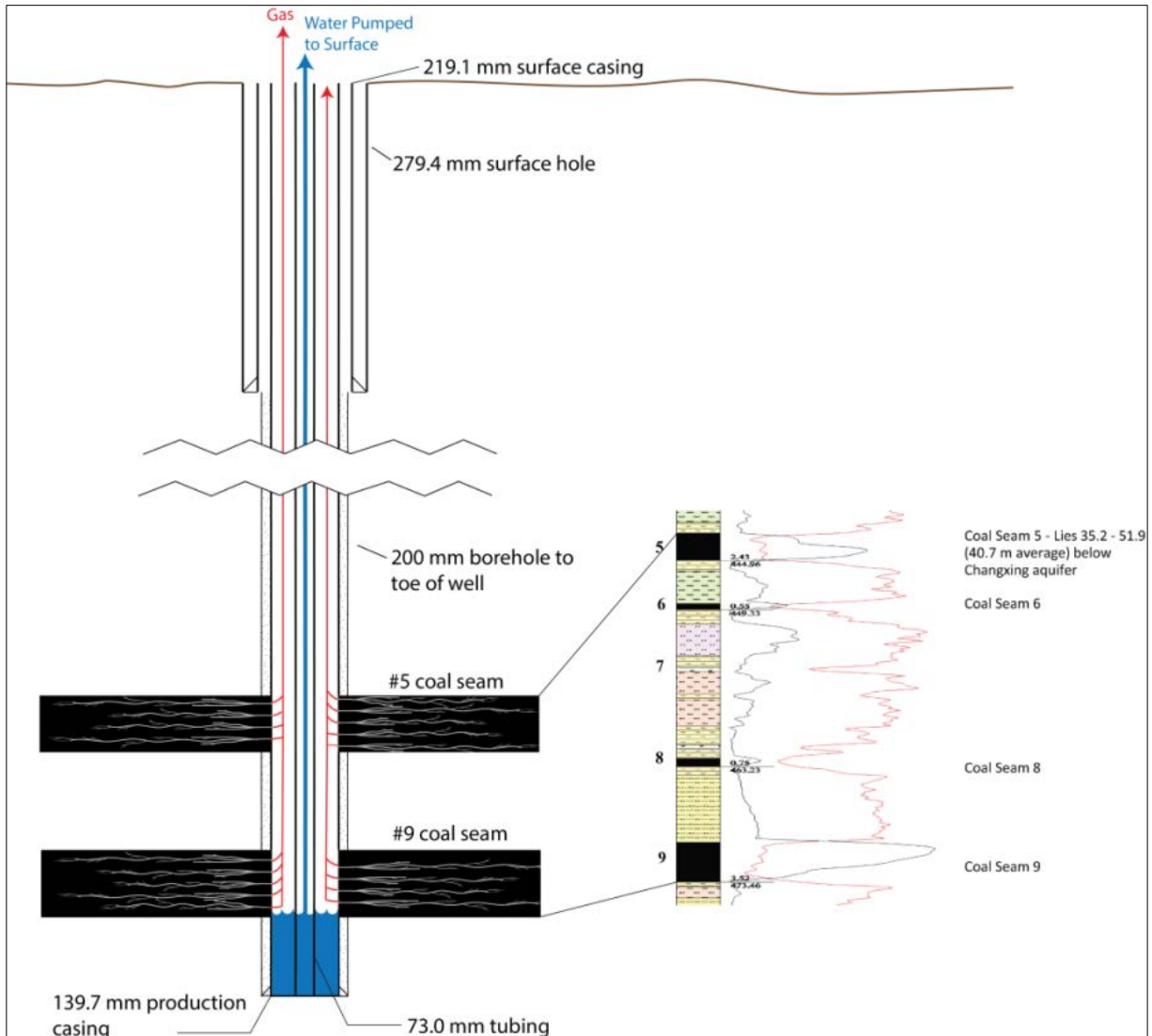
Figure 13: Pre-mine Well Diagram
