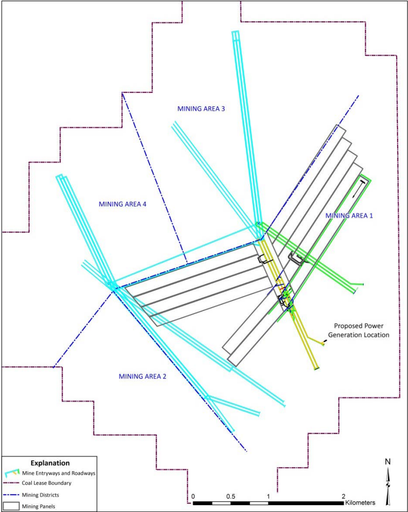
Figure 6: Mopanshan Mining Panels Map
