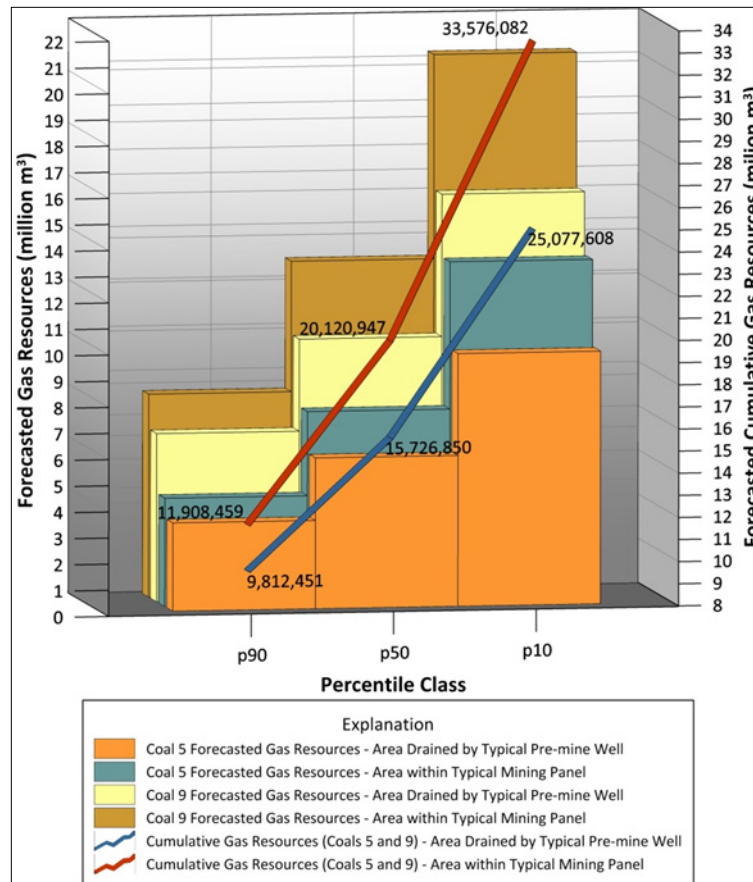
Figure 10: Forecasted Gas Resources - Typical Mining Panel and Area Drained by Pre-mine Well
