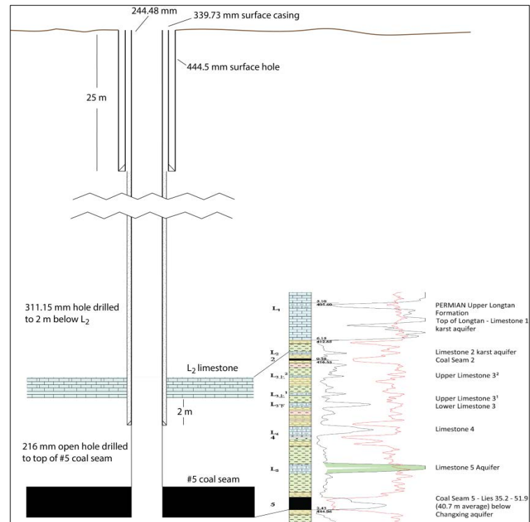
Figure 15: Example Proposed Gob Well
