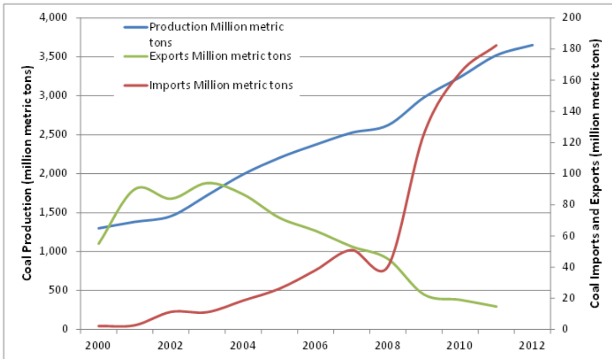
Figure 21: China's Raw Coal Supply. Source: EIA (2014b)
