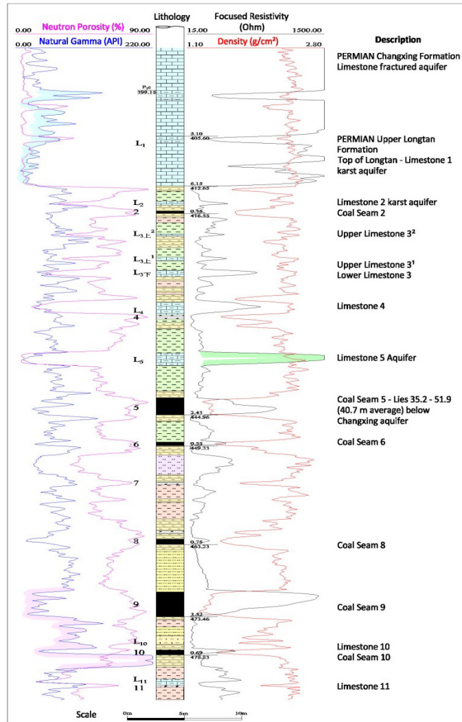
Figure 3: Stratigraphic Section of Coal and Water Bearing Strata
