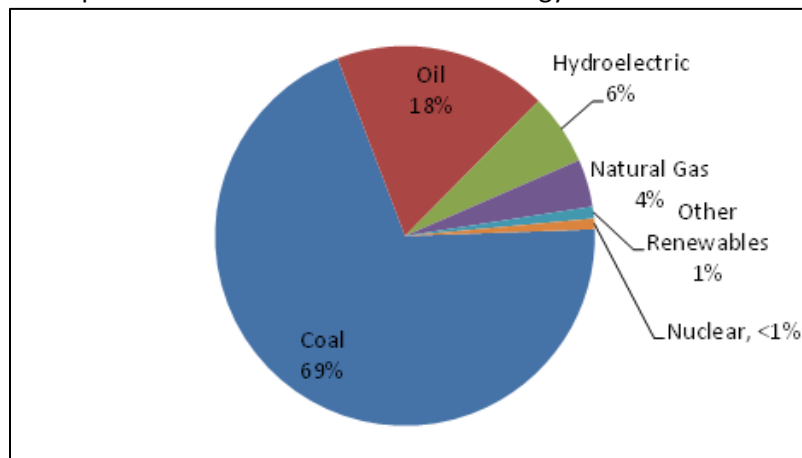
Figure 20: China's Energy Mix 2011. Source: EIA (2014a)
