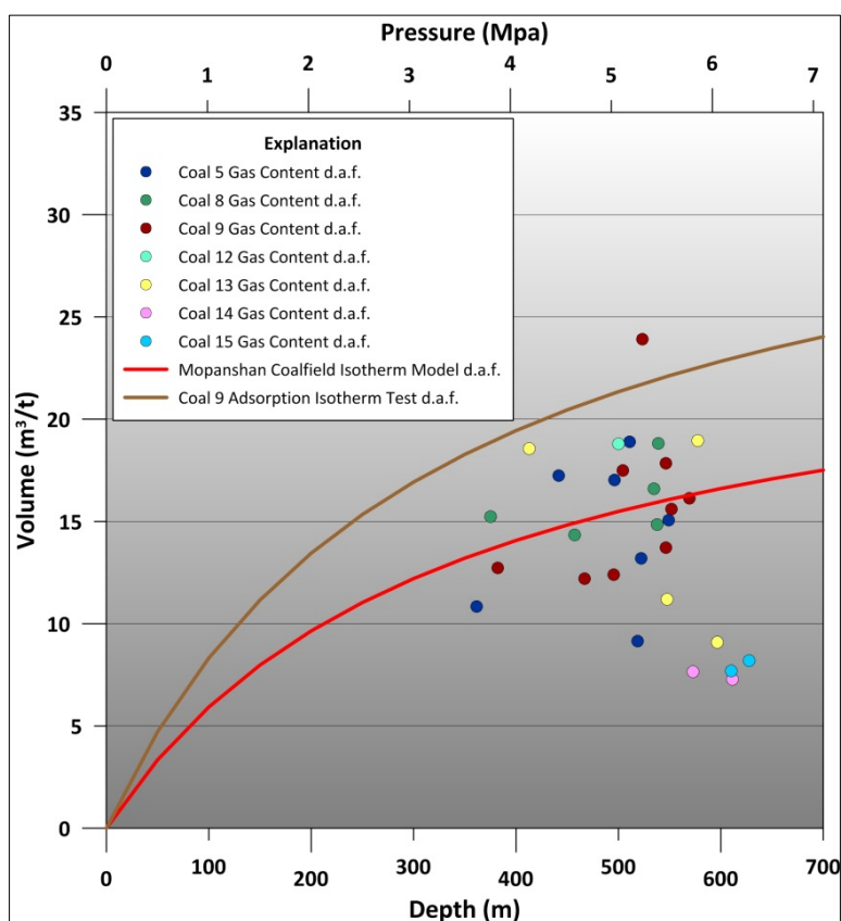
Figure 7: Adsorption Isotherm Curves and Gas Content Points
