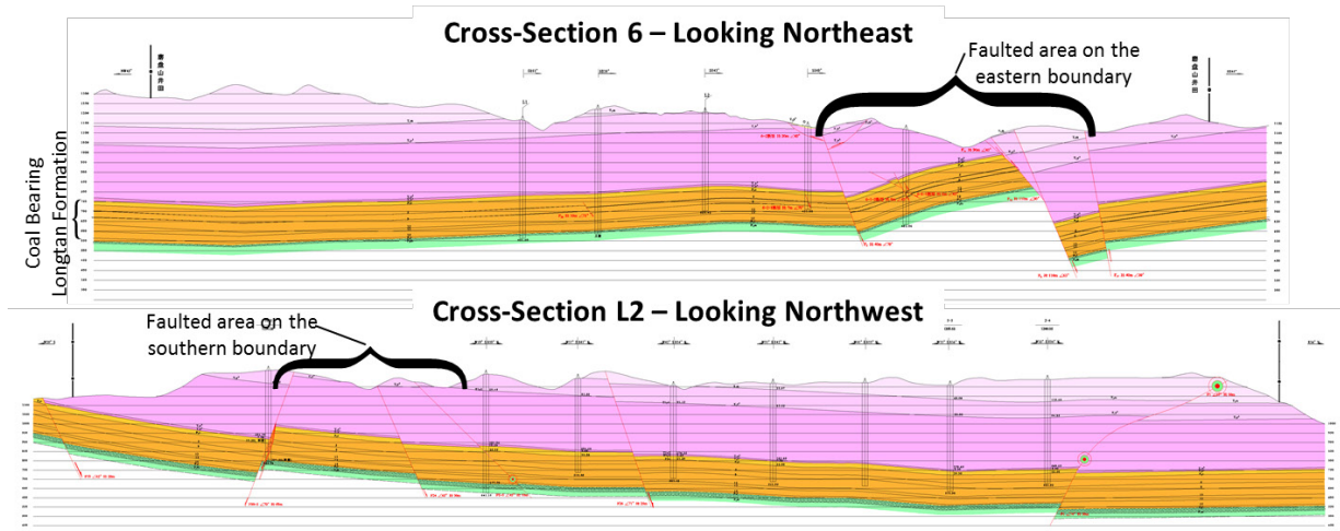
Figure 4: Example Cross-sections within the Mining Area
