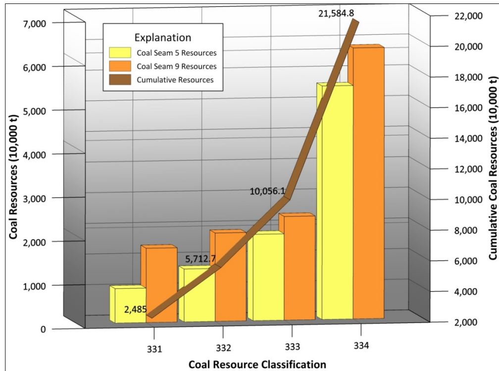
Figure 5: Seam 5 and Seam 9 Coal Resources
