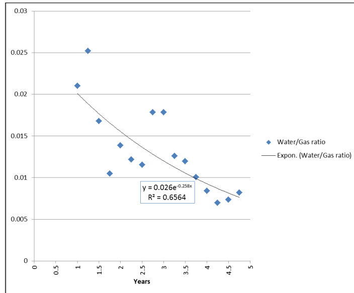
Figure 18: Water/Gas Ratio of Shouyang Production (cubic meters/cubic meters)
