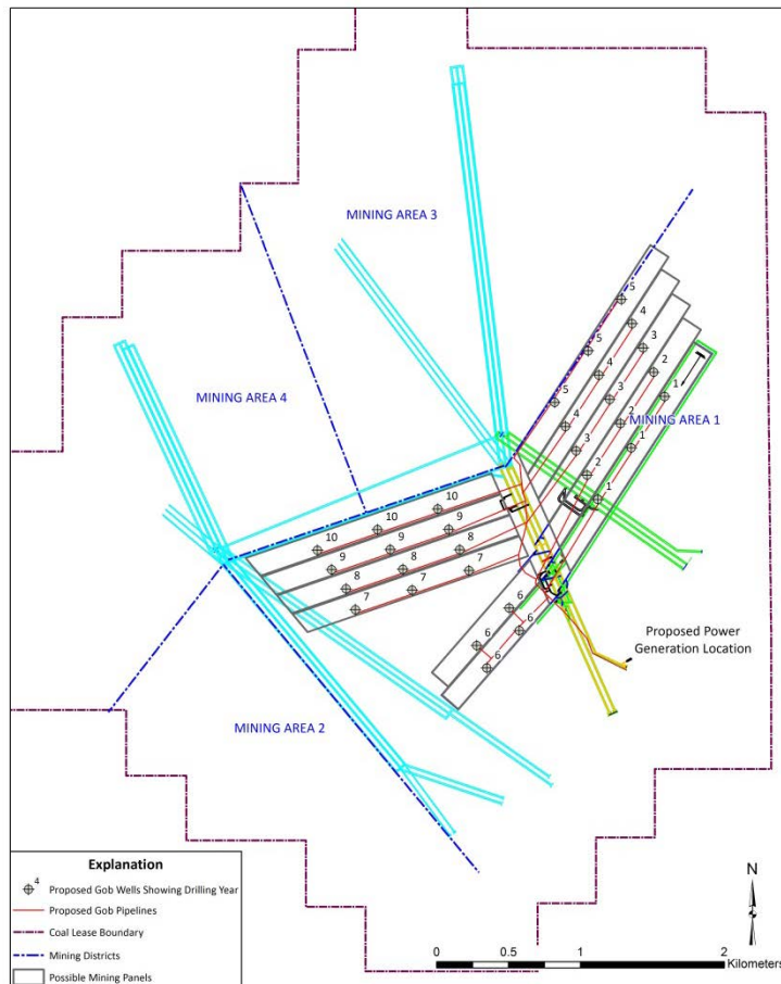
Figure 14: Layout of Proposed Gob Drainage Wells
