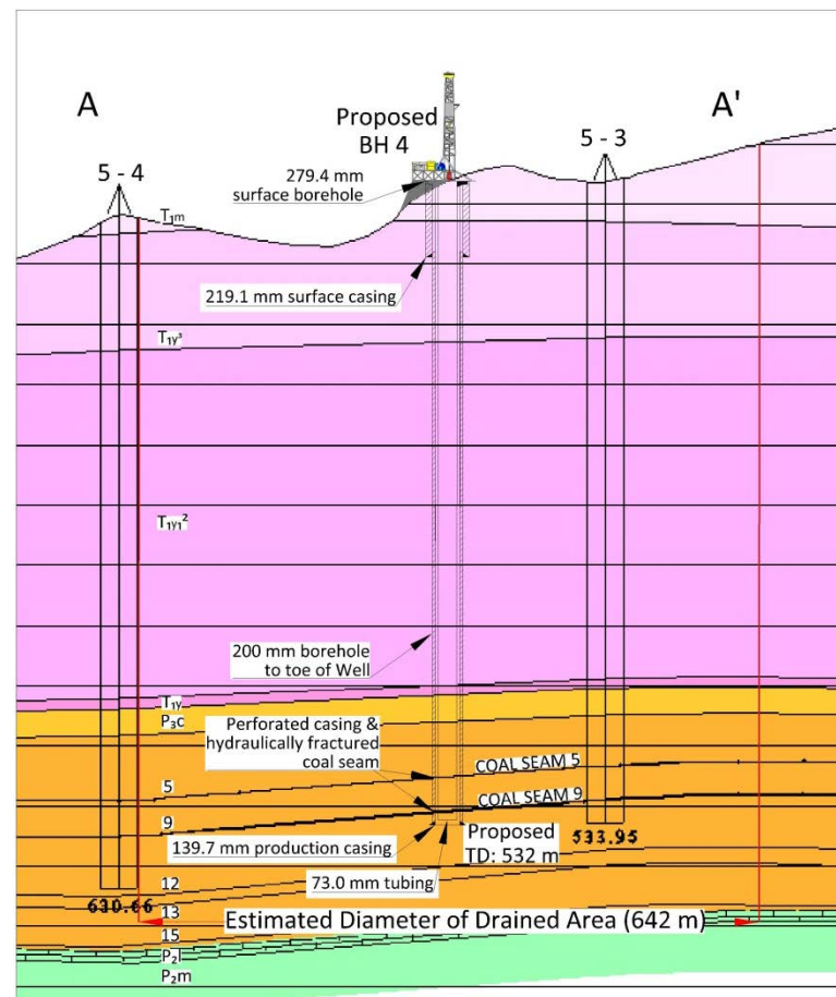
Figure 12: Example Proposed Pre-mine Well
