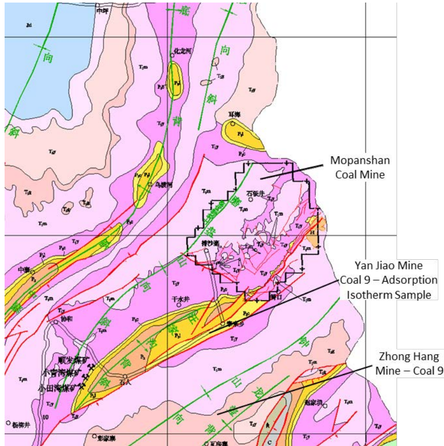
Figure 2: Mopanshan Regional Geologic Map
