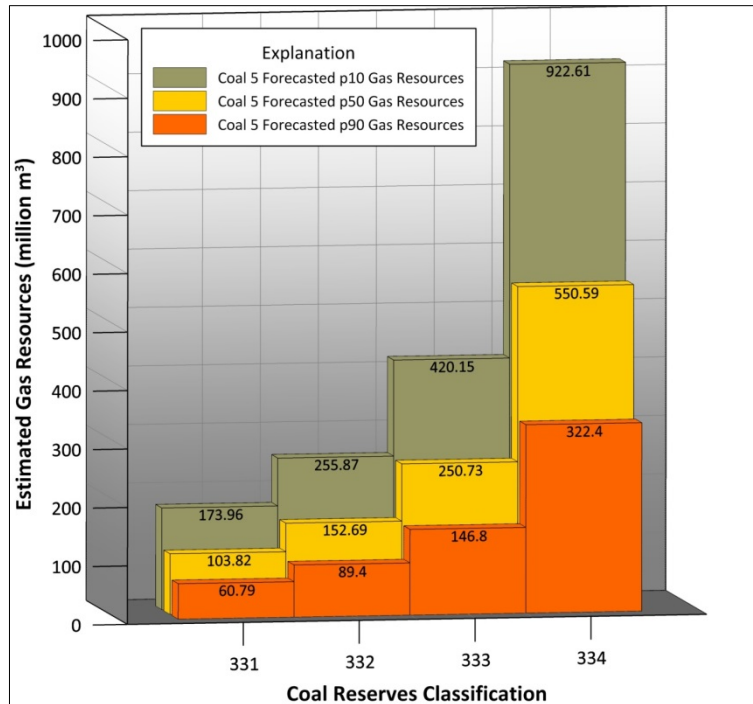
Figure 8: Coal Seam 5 Forecasted Gas Resources
