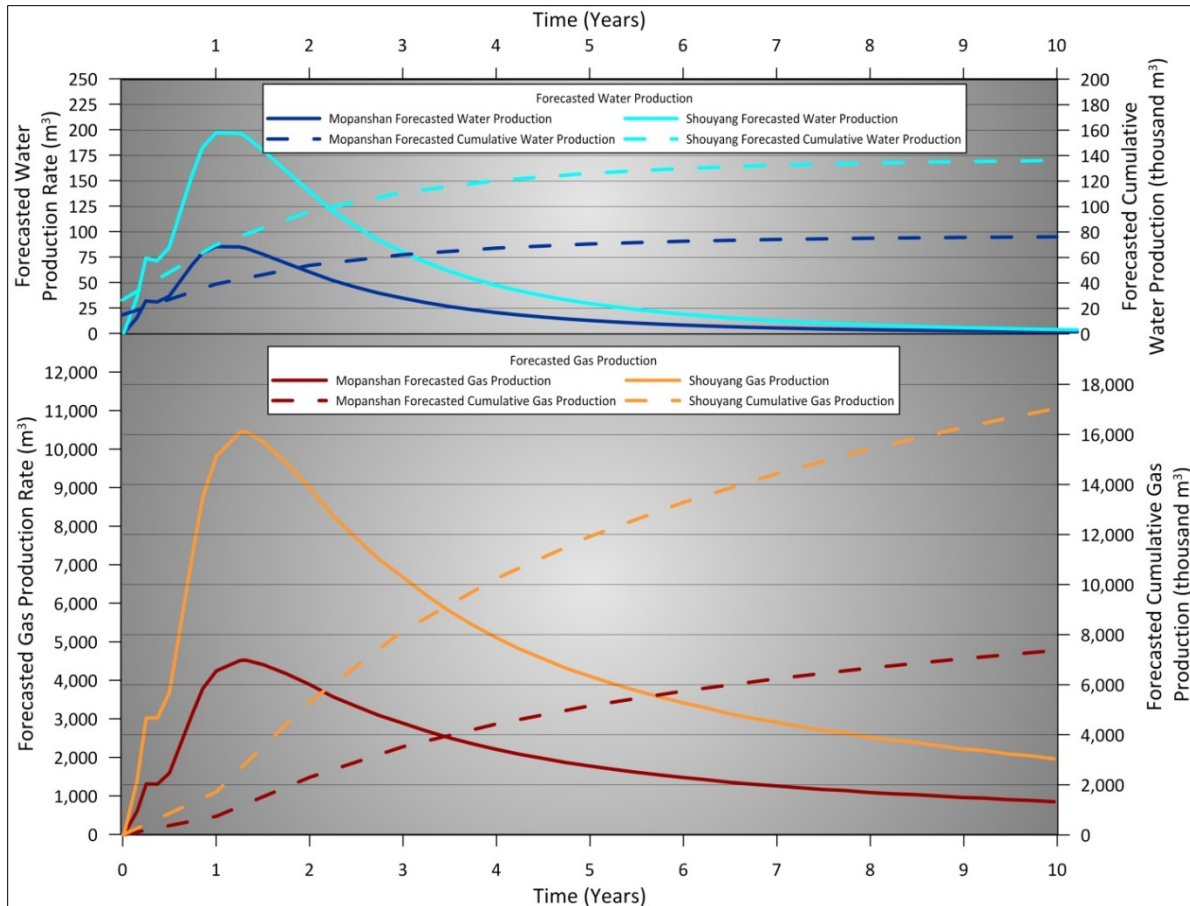
Figure 17: Forecasted Gas and Water Production - Comparing Mopanshan to Producing CBM Field
