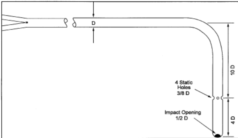
Figure 2C-1. Modified Hemispherical-Nosed Pitot Tube.
