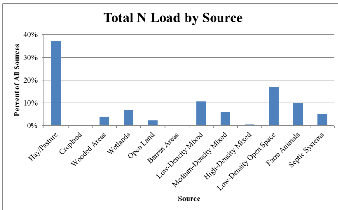
Figure 6: Total Nitrogen Load by Source in the Otter Brook Watershed
