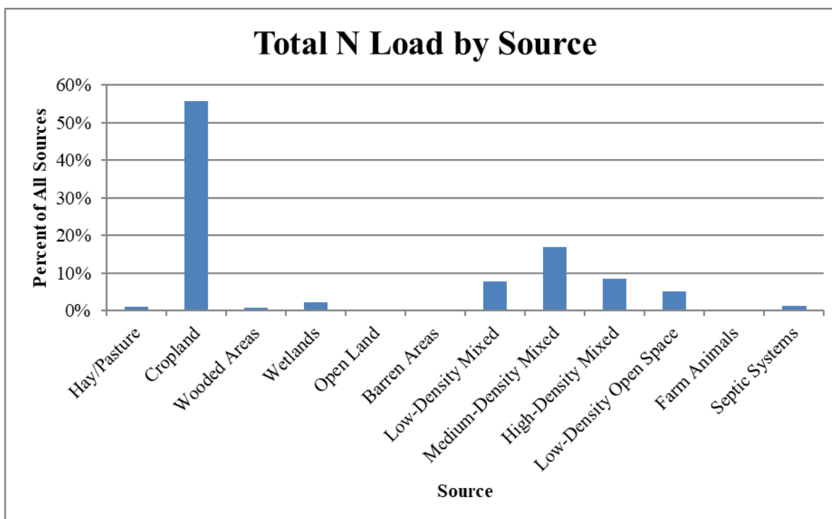
Figure 6: Total Nitrogen Load by Source in the Kennedy Brook Watershed
