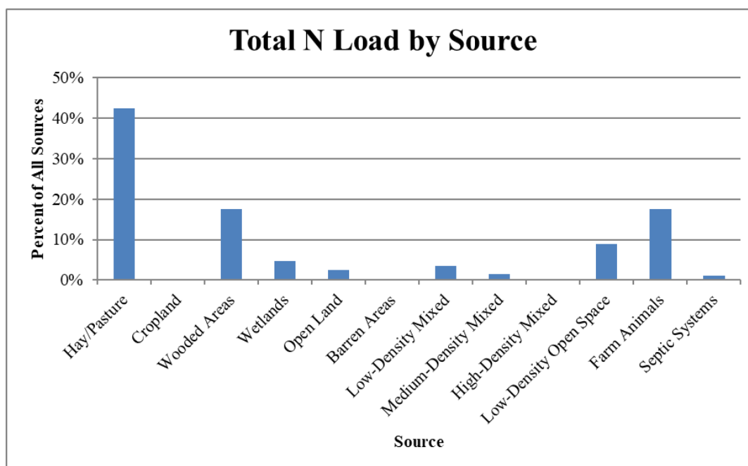
Figure 6: Total Nitrogen Load by Source in the Inkhorn Brook Watershed
