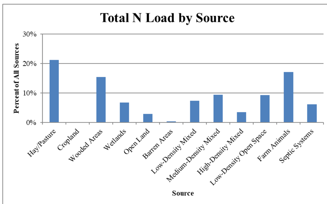
Figure 6: Total Nitrogen Load by Source in the Stetson Brook Watershed
