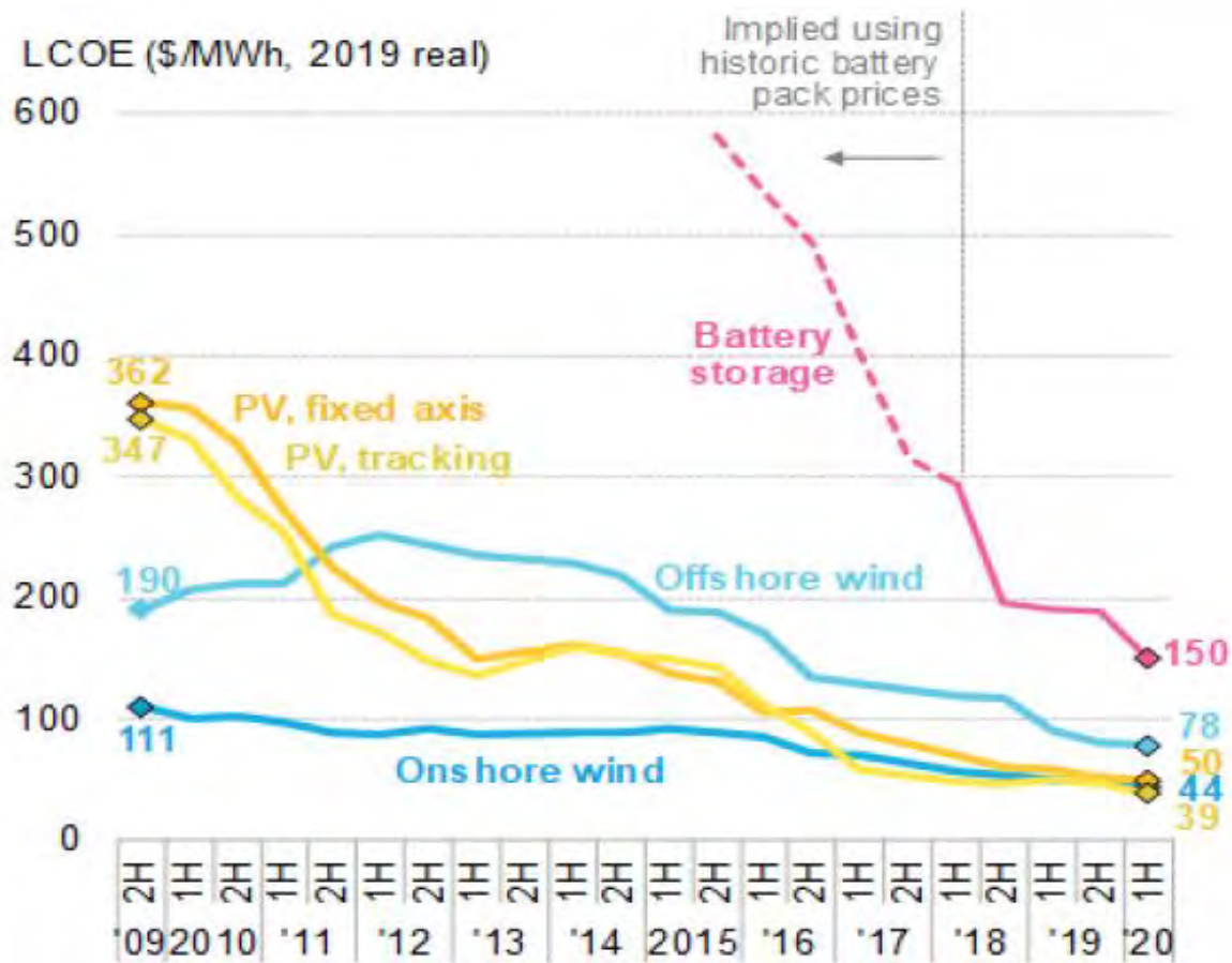
Figure 32. Global levelized cost of energy of battery storage technology relative to renewable energy generation technologies
