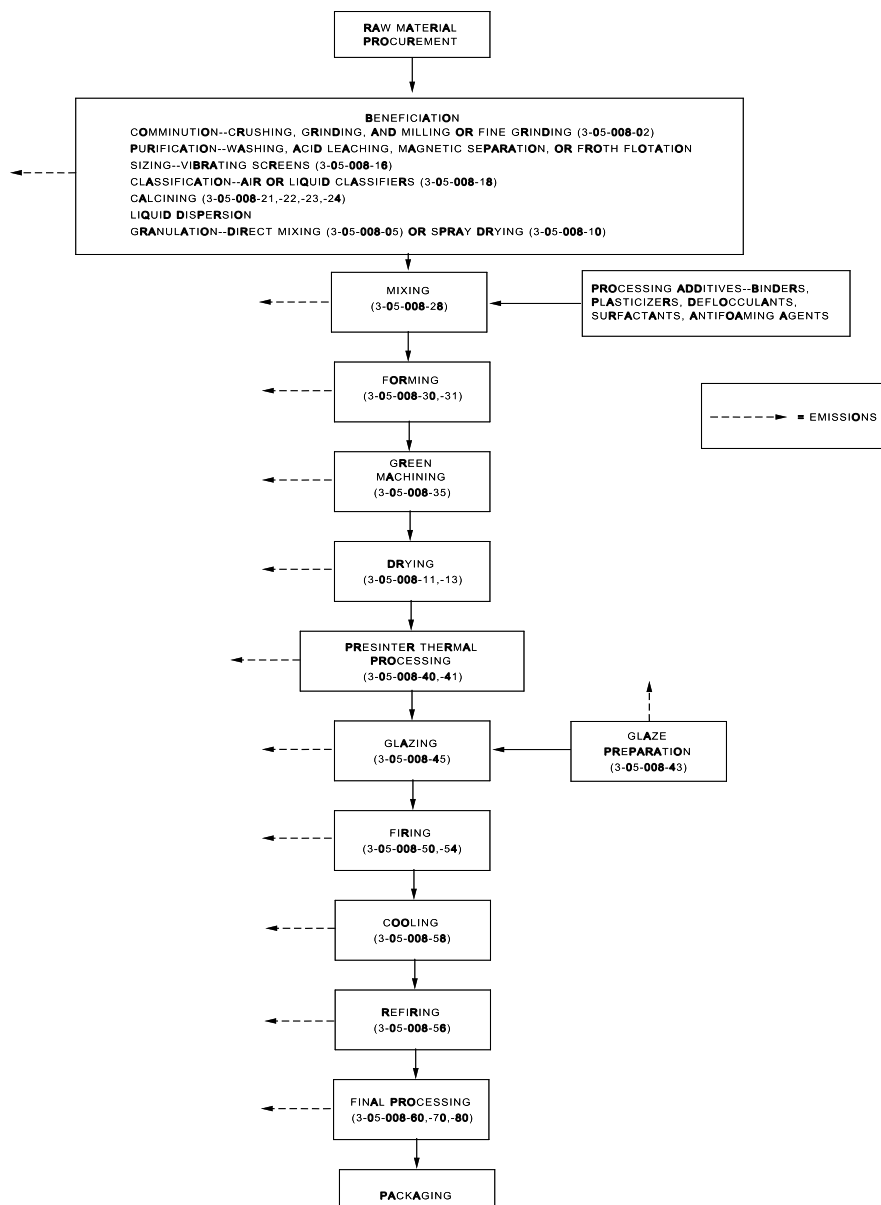
Figure 11.7-1. Process flow diagram for ceramic products manufacturing. (Source Classification Codes in parentheses.)
