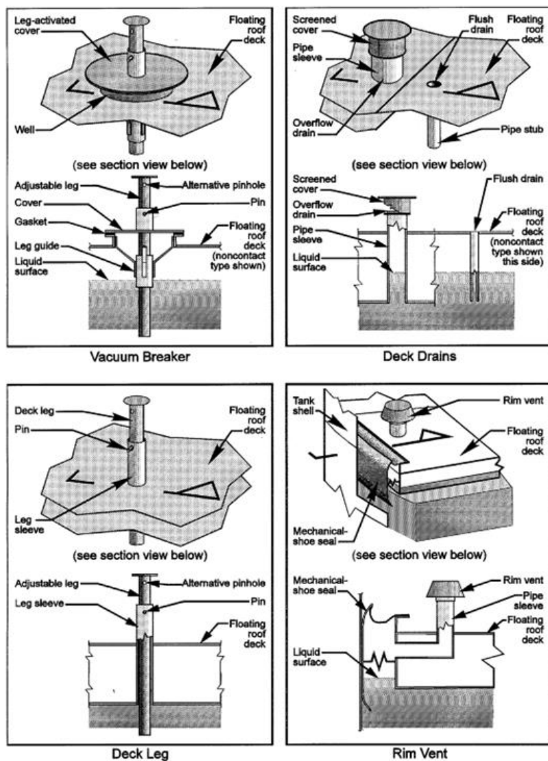
Figure 7.1-10. Deck fittings for floating roof tanks. 20
