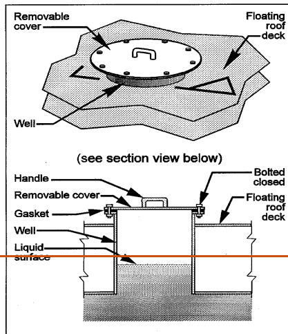
Access Hatch
