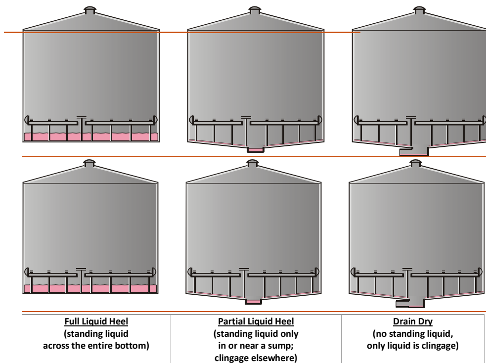
Figure 7.1-20. Bottom conditions for landing loss. 20
