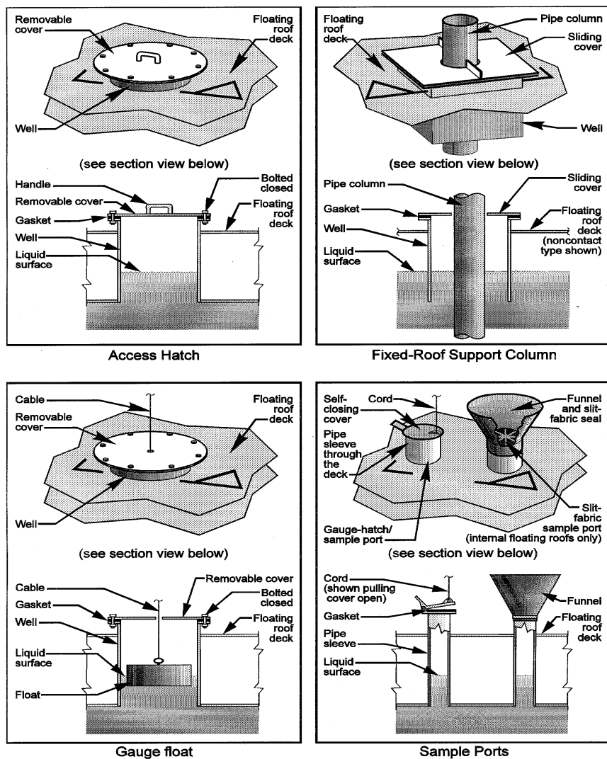
Figure 7.1-9. Deck fittings for floating roof tanks. 20
