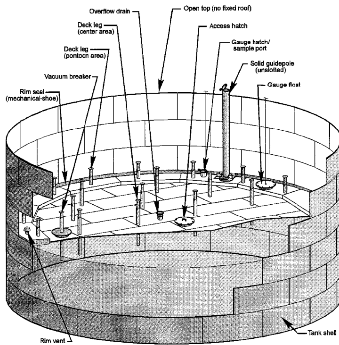
Figure 7.1-2. External floating roof tank (pontoon type) 20
