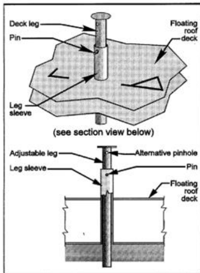
Deck Leg
