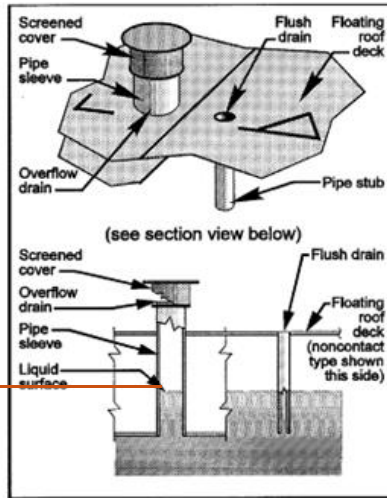
Deck Drains
