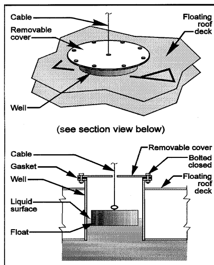
Gauge float
