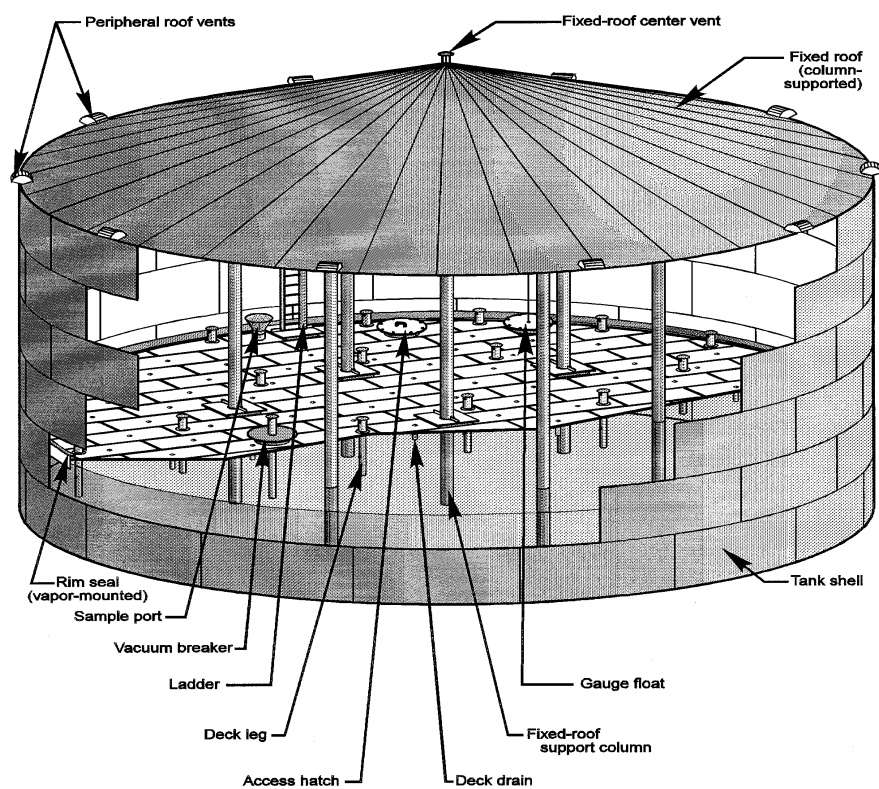
Figure 7.1-4. Internal floating roof tank. 20
