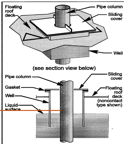
Fixed-Roof Support Column
