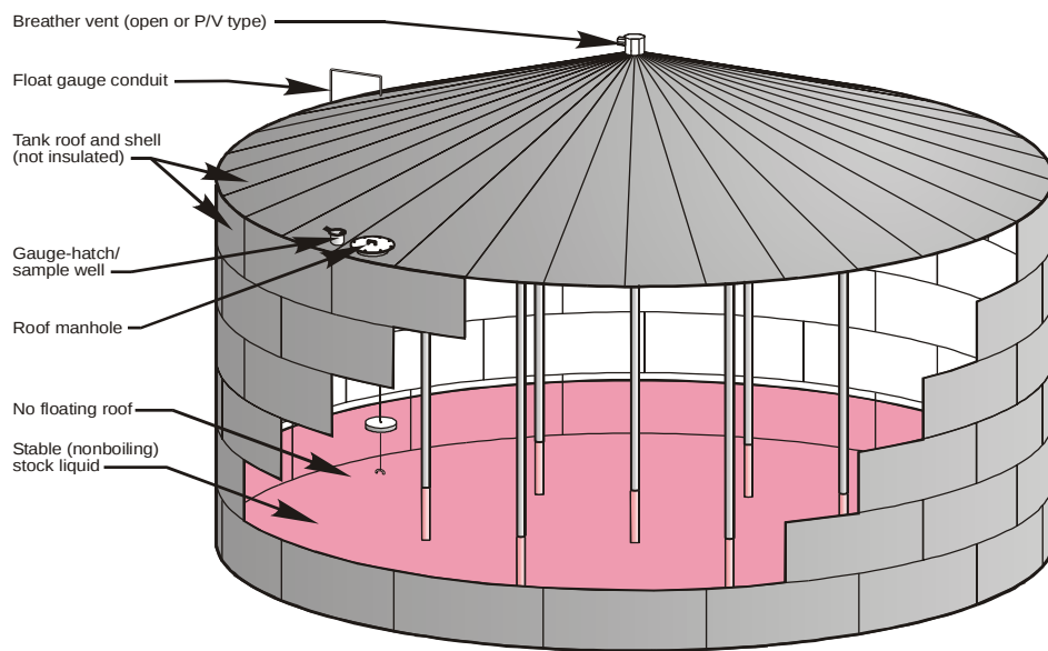
Figure 7.1-1. Typical fixed-roof tank. 20
