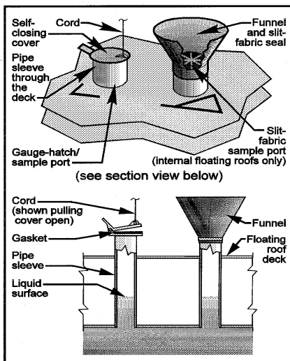
Sample Ports
