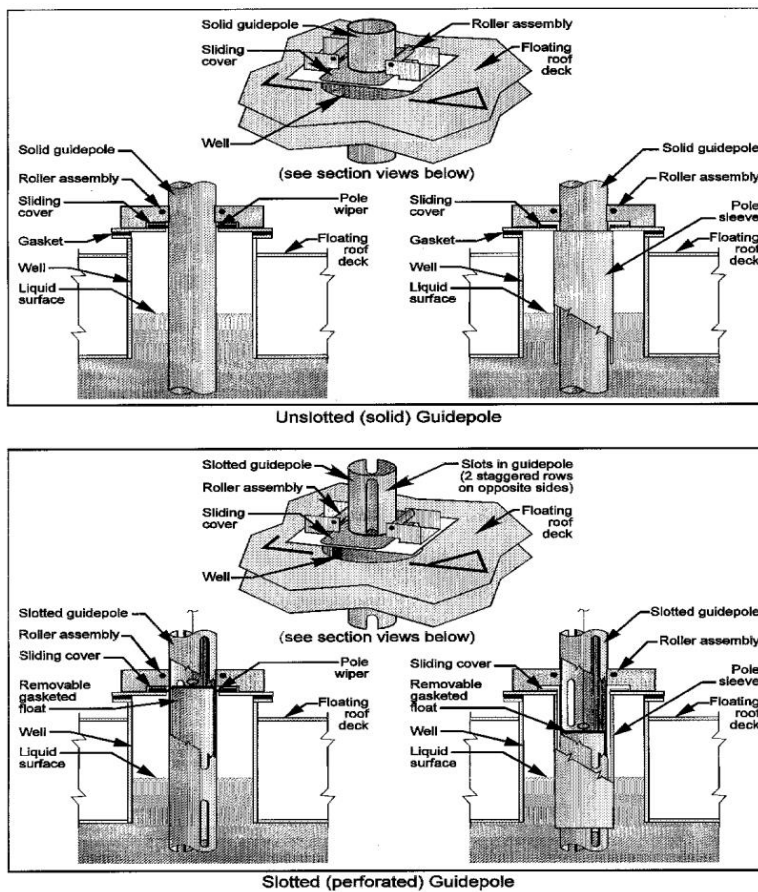
Figure 7.1-11. Slotted and unslotted guidepoles. 20
