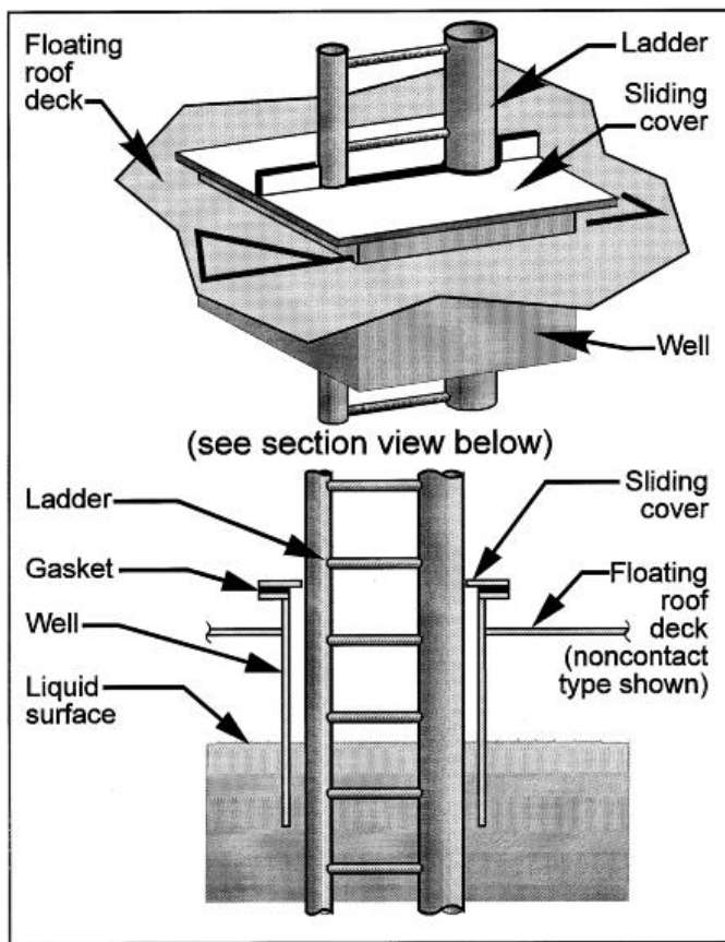
Figure 7.1-12. Ladder well. 20
