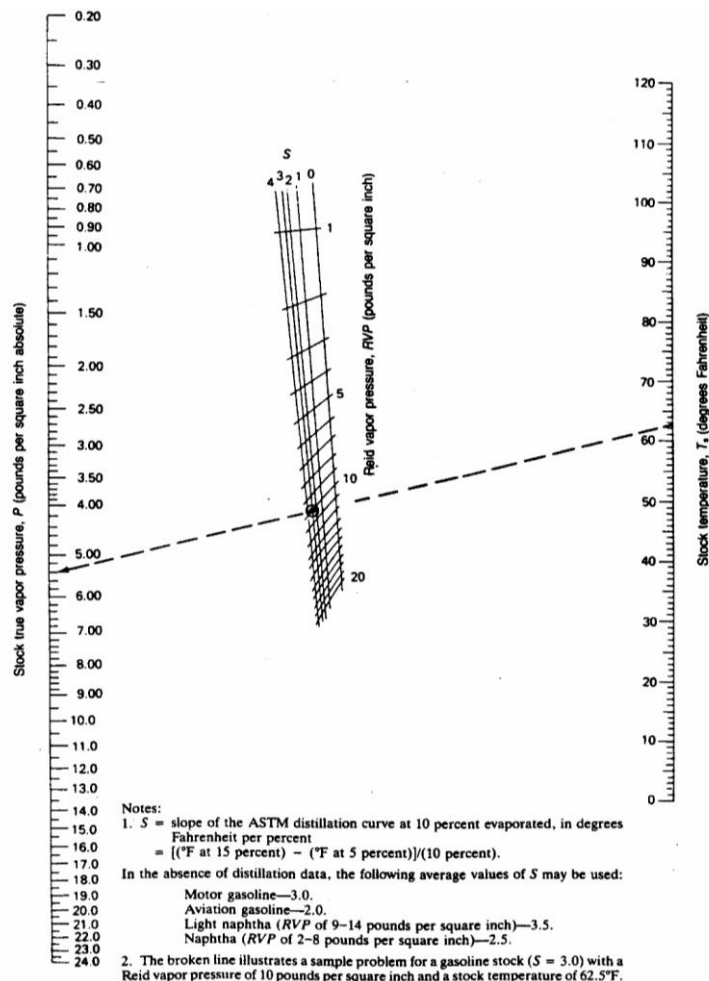
Figure 7.1-14a. True vapor pressure of refined petroleum stocks with Reid vapor pressures of 1 to 20 psi. 4
