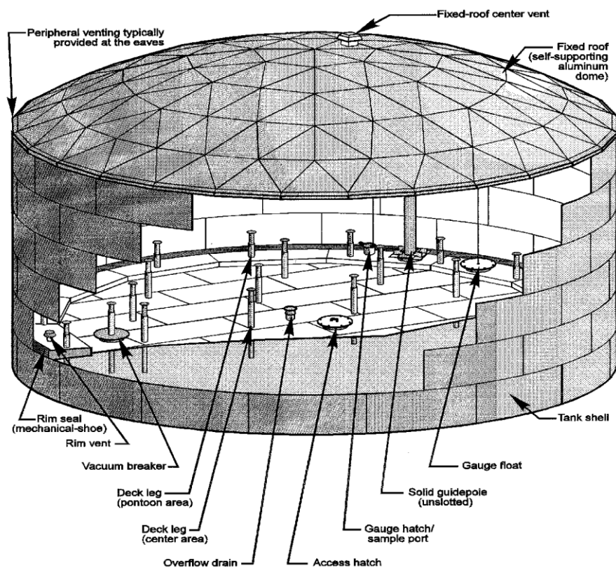
Figure 7.1-5. Domed external floating roof tank. 20
