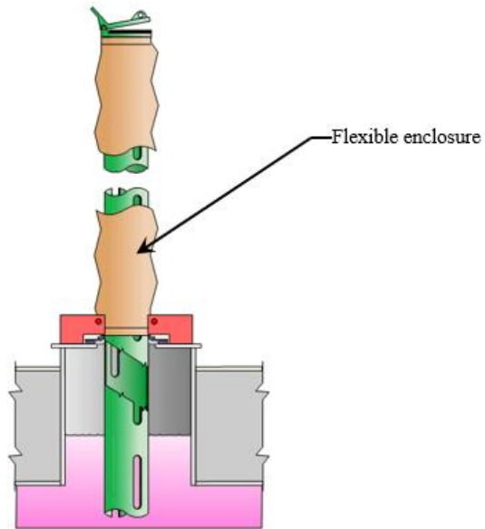
Figure 7.1-22. Slotted-guidepole with flexible enclosure. 20
