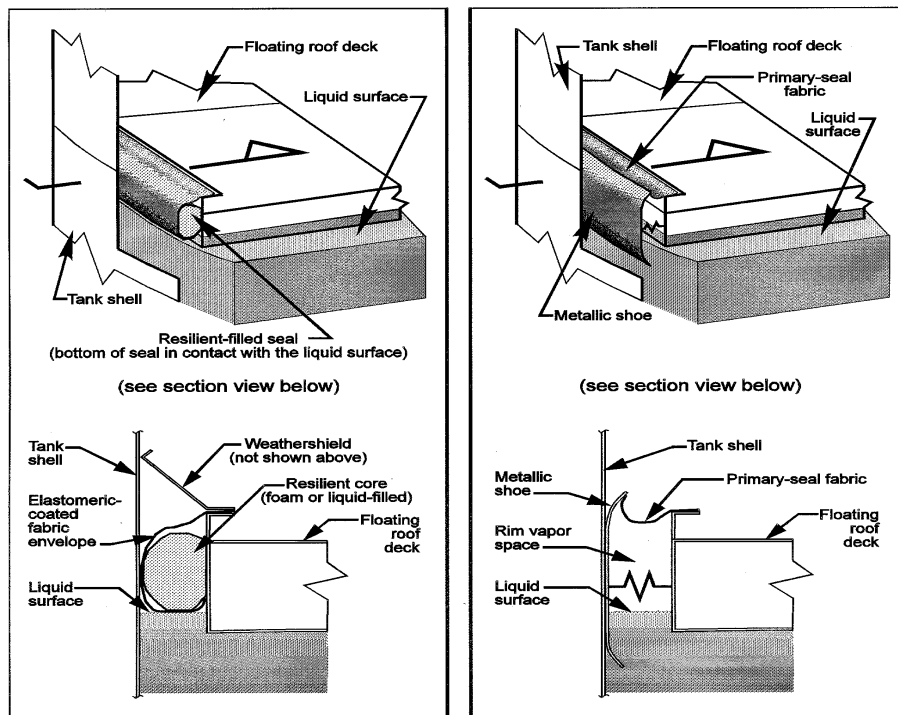
Figure 7.1-7. Liquid-mounted and mechanical shoe primary seals. 20
