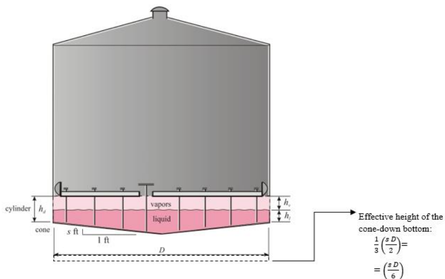
Figure 7.1-23. Height of the liquid heel and vapor space under a landed floating roof. 20 This figure illustrates variables used in Table 7.1-4.
