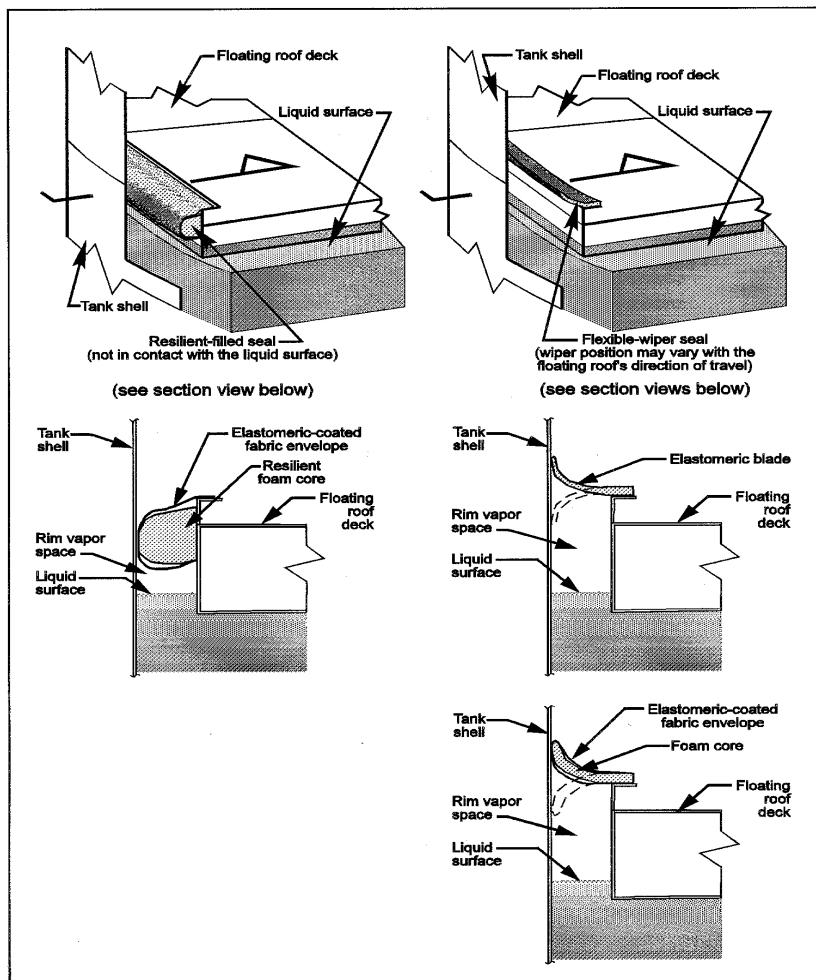
Figure 7.1-6. Vapor-mounted primary seals. 20
