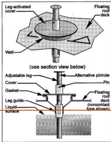
Vacuum Breaker
