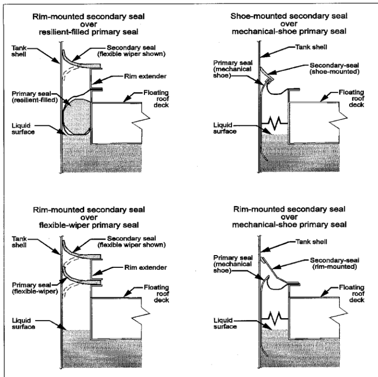
Figure 7.1-8. Secondary rim seals. 20
