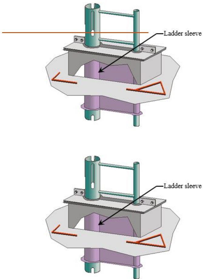
Figure 7.1-21. Ladder-slotted guidepole combination with ladder sleeve. 20
