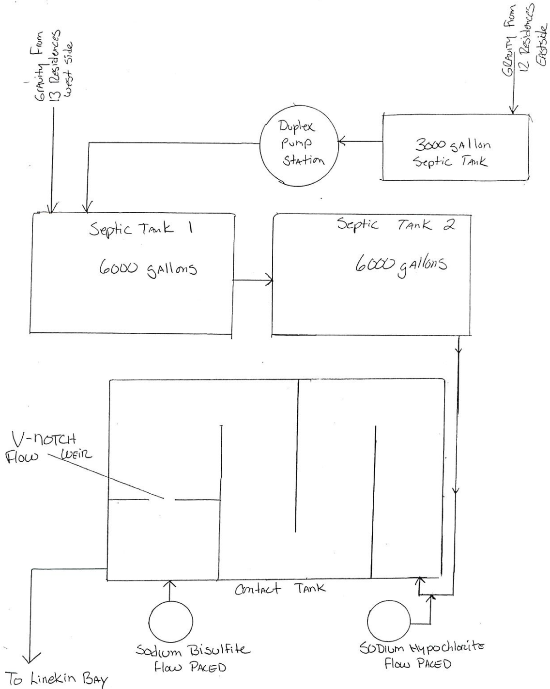
Figure 2 – Flow Schematic
