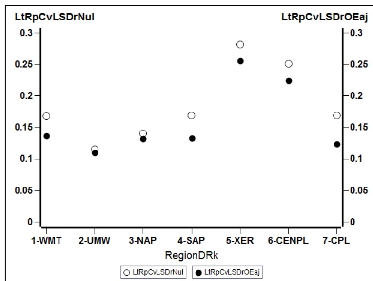
Figure 5-4. \text{LogSD} 's for Null-Model and regression-based O/E model for Near-shore RVegQ , LitCvrQ , and LitRipCvrQ in the set of least-disturbed lakes and reservoirs (Table 5-1) sampled in the combined 2007 and 2012 NLA surveys.
