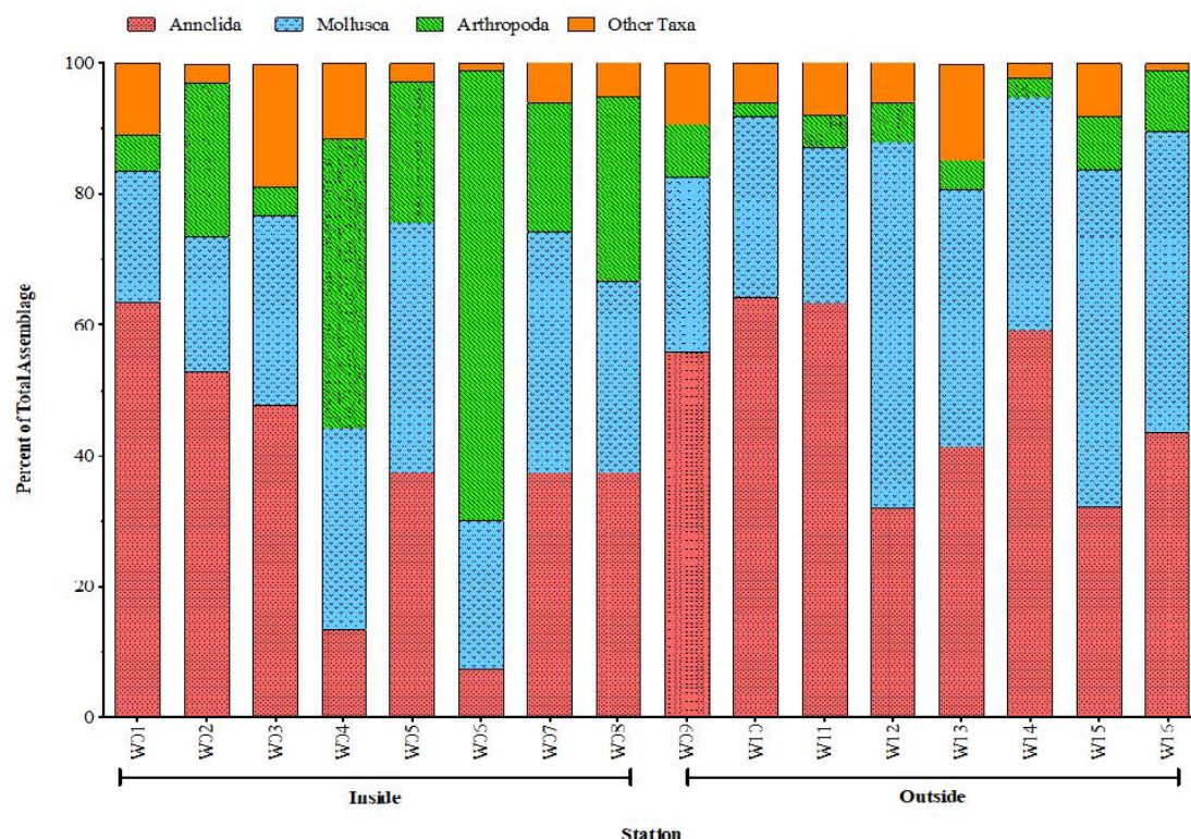
Figure 19. 2020 distribution of major taxonomic groups at the Wilmington ODMDs.
