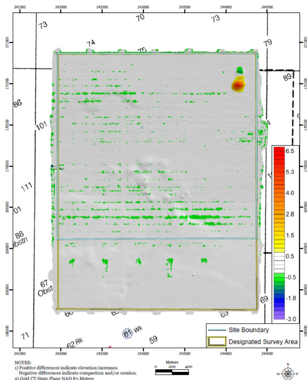
Figure 5. WLDS bathymetric elevation comparison (depth difference) 2020 vs 2014. Positive differences between surveys suggest deposition/accretion since 2014 (indicated in yellow, orange, and red); negative differences suggest compaction/erosion since 2014 (indicated in green).
