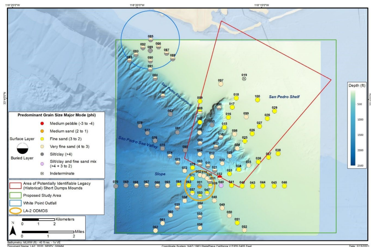
Figure 26. Predominant grain size by station in the LA-2 study area. Most stations are characterized by soft sediments.
