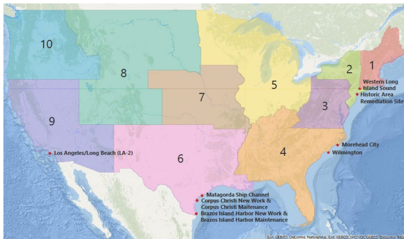
Figure 1. Approximate locations of the ten ocean sites surveyed in 2020. Numbers indicate EPA Regions.
