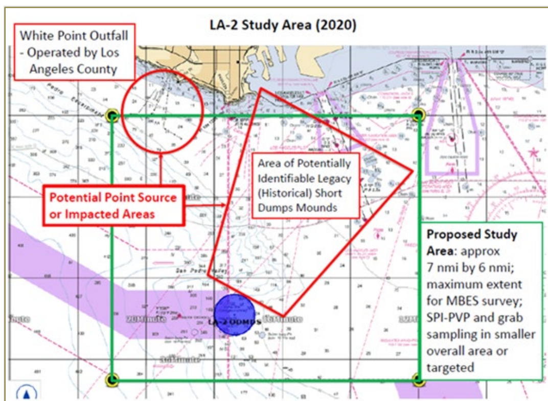
Figure 24. LA-2 ODMDS and study area offshore of Los Angeles-Long Beach, CA.
