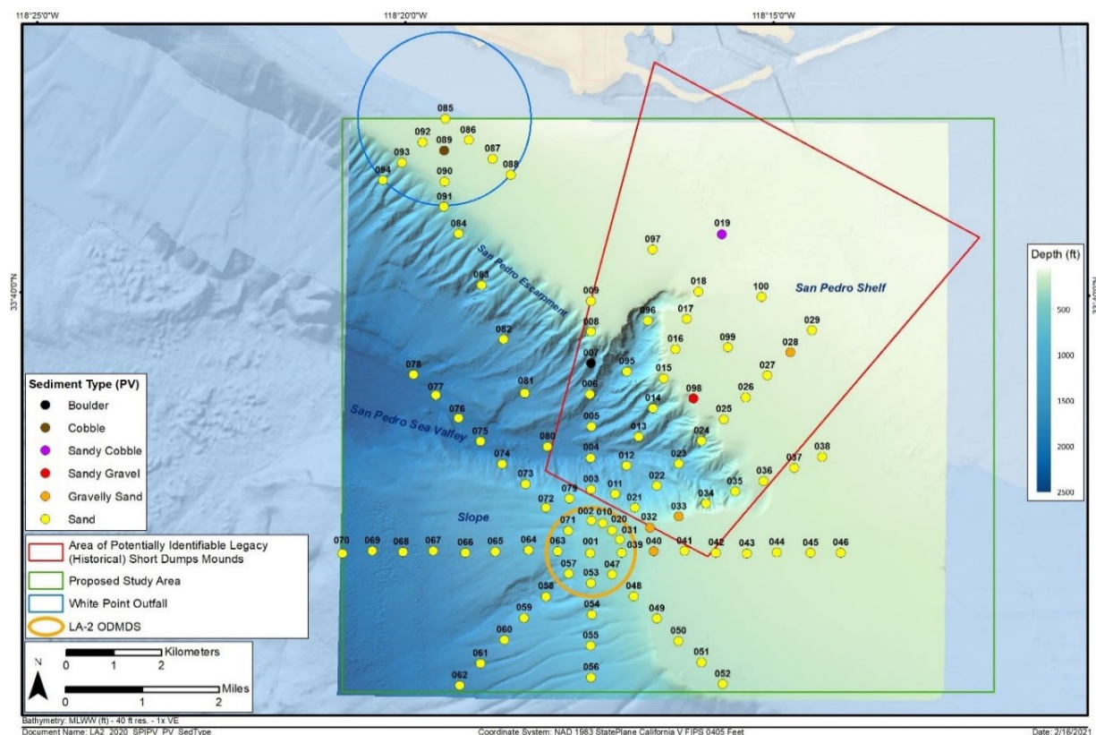
Figure 27. Sediment type derived from PVI analysis denoting presence of gravels at the LA-2 study area.
