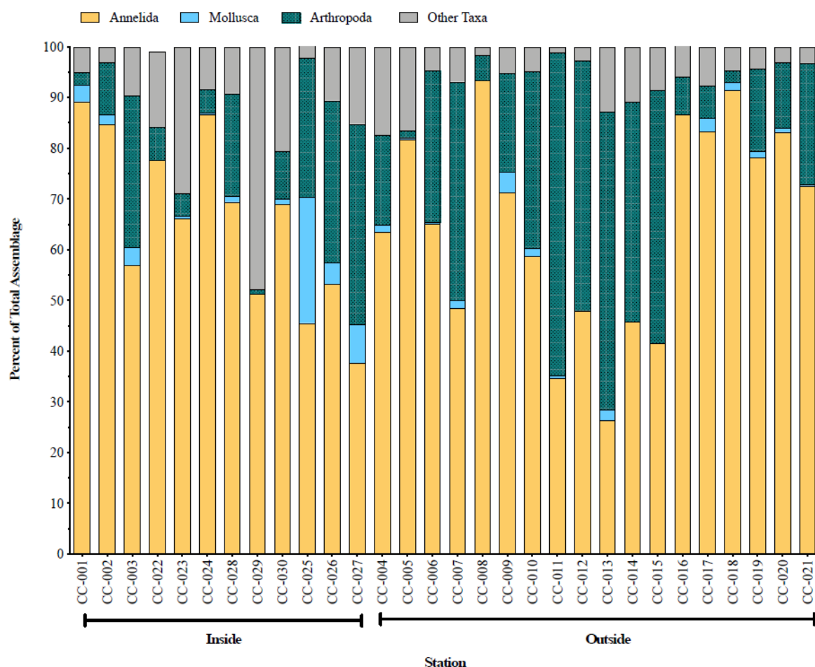
Figure 19. Distribution of major taxa for the Corpus Christi, Texas sampling stations, 2020.
