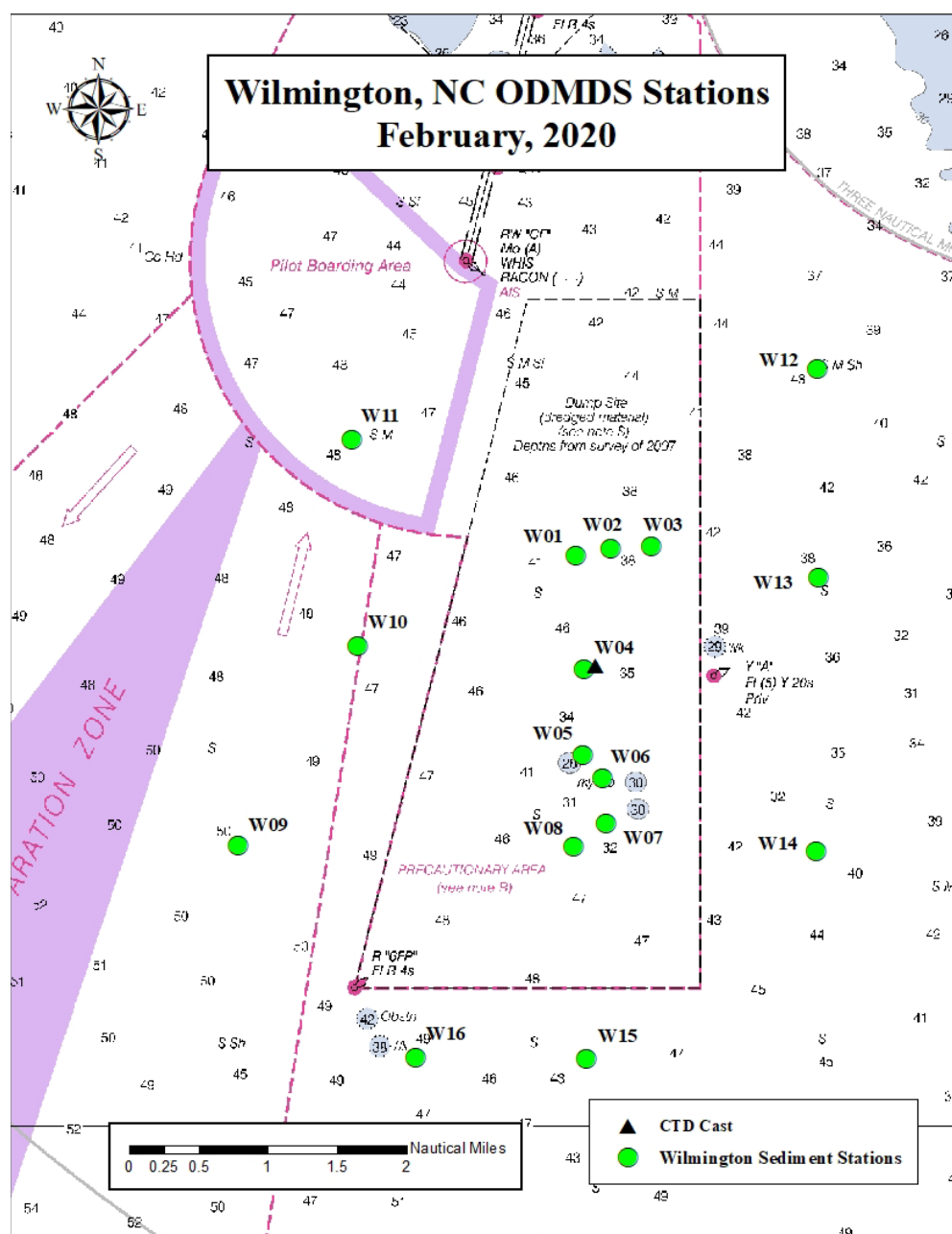
Figure 12. Wilmington ODMDS and sampling stations. Sixteen stations were sampled for sediment chemistry and macroinvertebrates, eight of which were outside the ODMDS (W09-W16).
