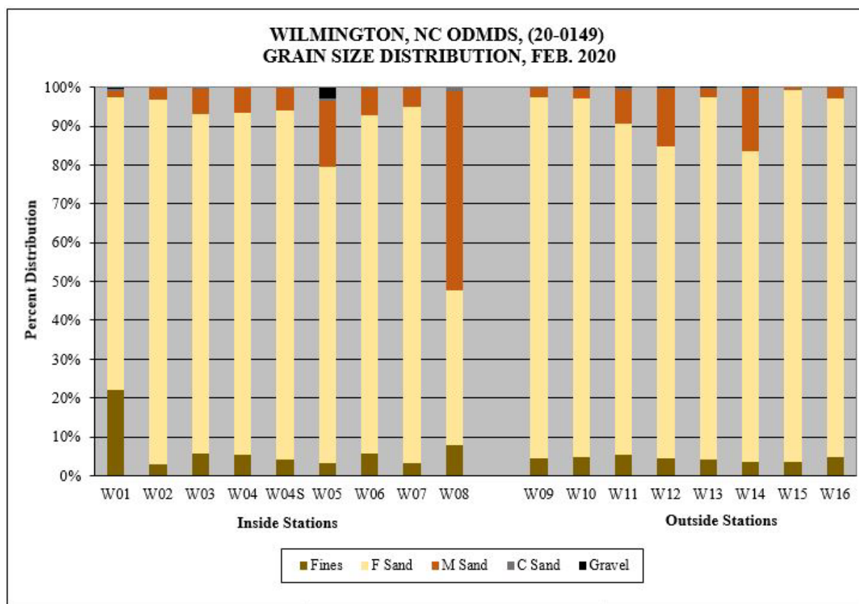
Figure 13. Grain size distribution at the Wilmington ODMDS. Sediment grain sizes were similar at stations both inside and outside the ODMDS.
