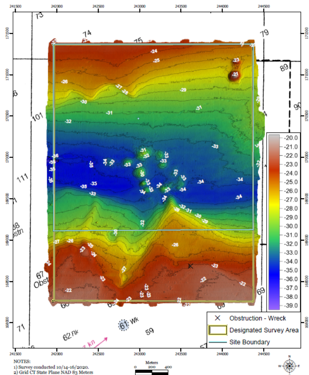
Figure 4. Bathymetry of the study area, including the WLDS, as measured during the 2020 survey.
