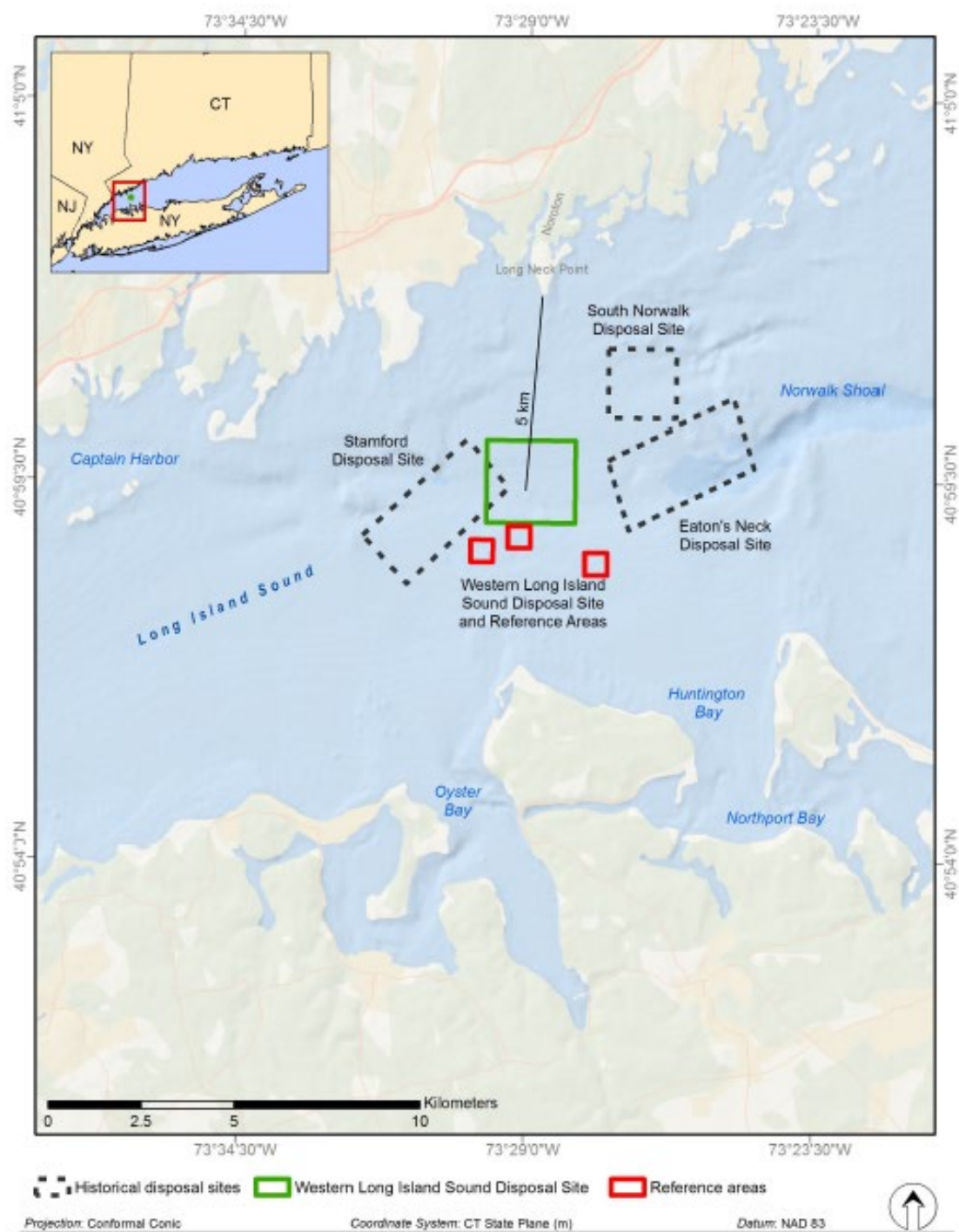
Figure 2. Location of the Western Long Island Sound Disposal Site (WLDS), depicted as the green square. The red squares are reference areas, which are sampling locations used for comparison when evaluating WLDS conditions.
