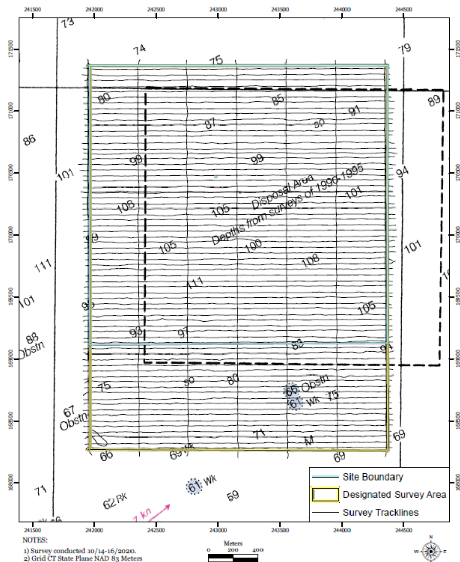
Figure 3. Acoustic survey transects at the WLDS disposal site. Survey lines are 148 ft (45 m) apart with crosslines spaced 1,312 ft (400 m) apart, with a total length of 123.4 miles (198.6 km).
