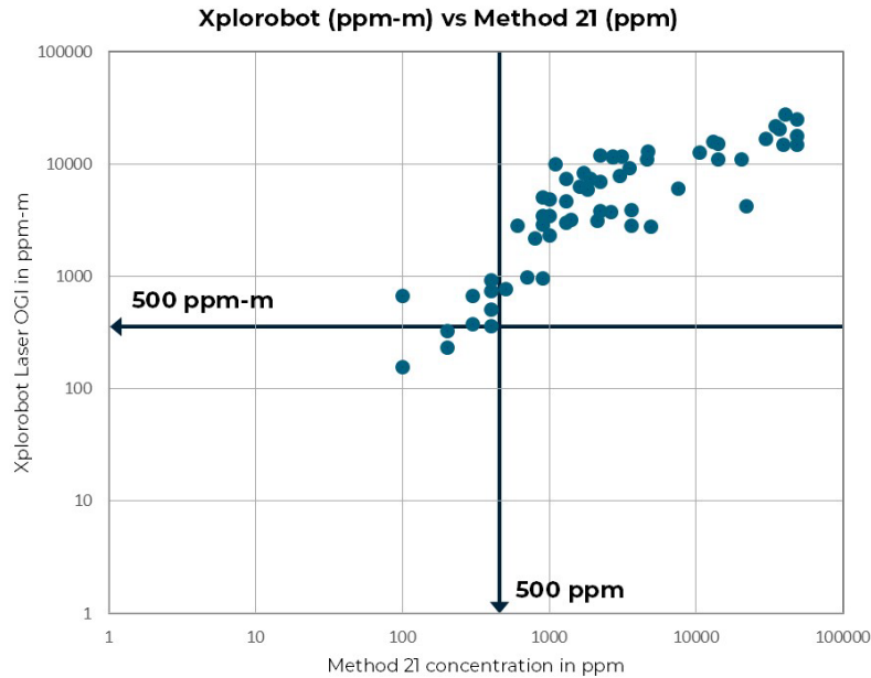
Figure 4. Comparison between Xplorobot Laser Gas Imager and Method 21 device measurements. In controlled rate experiments the 500-ppm measurement on a Method 21 device (closer than 1 m in distance) corresponded to a 500 ppm-m measurement of Xplorobot Laser Gas Imager (from distances between 1 and 5 m).
