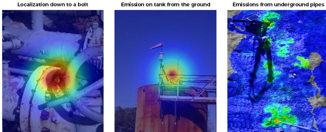
Figure 1. Examples of methane emission visualization using Xplorobot Laser Gas Imager. On the left is methane emission visualization for a leak from a bolt on a flange. In the center is methane emission visualization for leak from a thief hatch on a tank. On the right is methane emission visualization for leak from an underground pipeline.
