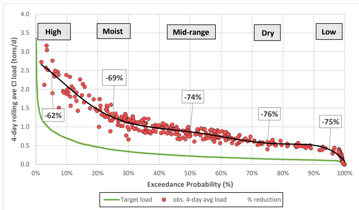
FIGURE 12: OBSERVED AND TARGET CHLORIDE LOAD DURATION CURVES FOR SUNNYSIDE BROOK BASED ON FOUR-DAY ROLLING AVERAGES, INCLUDING PERCENT REDUCTIONS CALCULATED FOR THE PERCENTILE MID-POINT OF THE HIGH, MOIST, MID-RANGE, DRY AND LOW STREAMFLOW CATEGORIES.
