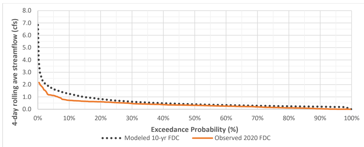
FIGURE 9: OBSERVED AND MODELED FLOW DURATION CURVES BASED ON FOUR-DAY AVERAGE STREAMFLOW.
