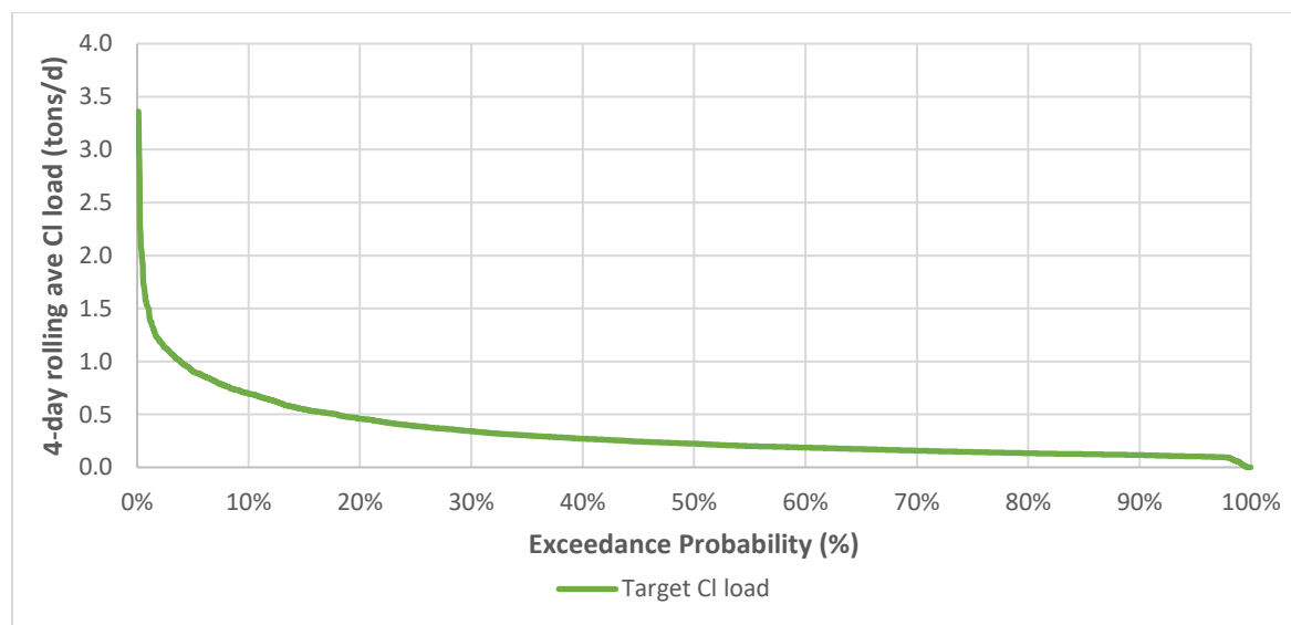
FIGURE 11: TARGET LOAD DURATION CURVE FOR SUNNYSIDE BROOK, DERIVED FROM FOUR-DAY ROLLING AVERAGE CHLORIDE LOADS BASED ON 90% OF THE VERMONT CHRONIC CHLORIDE WATER QUALITY STANDARD.
